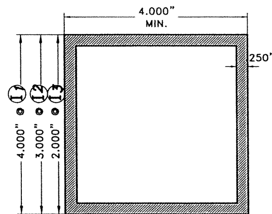
(I, I2, I3) BUILD-OUT MOUNTED TUBE (MASONRY) 6061-T6 ALUMINUM ALLOY TEMPER
