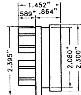
RIGHT VIEW
