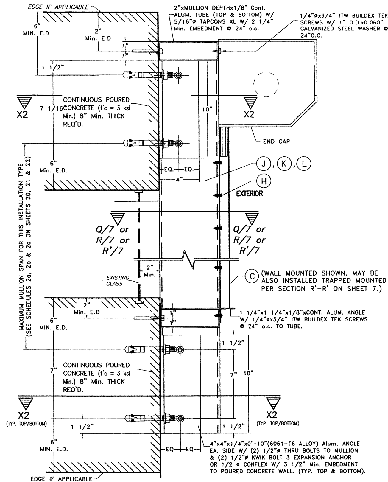
SECTION X2-X2 W/ (J), (K) or (L)* (END & INTERIOR MULLION (J), (K) or INTERIOR MULLION (L) (W/ ORIENTATION # 2) (6"x4" , 8"x4" or 4"x4")
