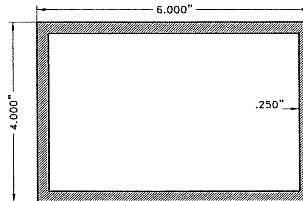
(J) 4" x 6" MULLION 6061-T6 ALUMINUM ALLOY TEMPER
