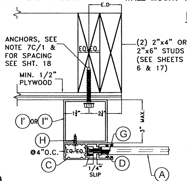
BUILD-OUT MOUNT
