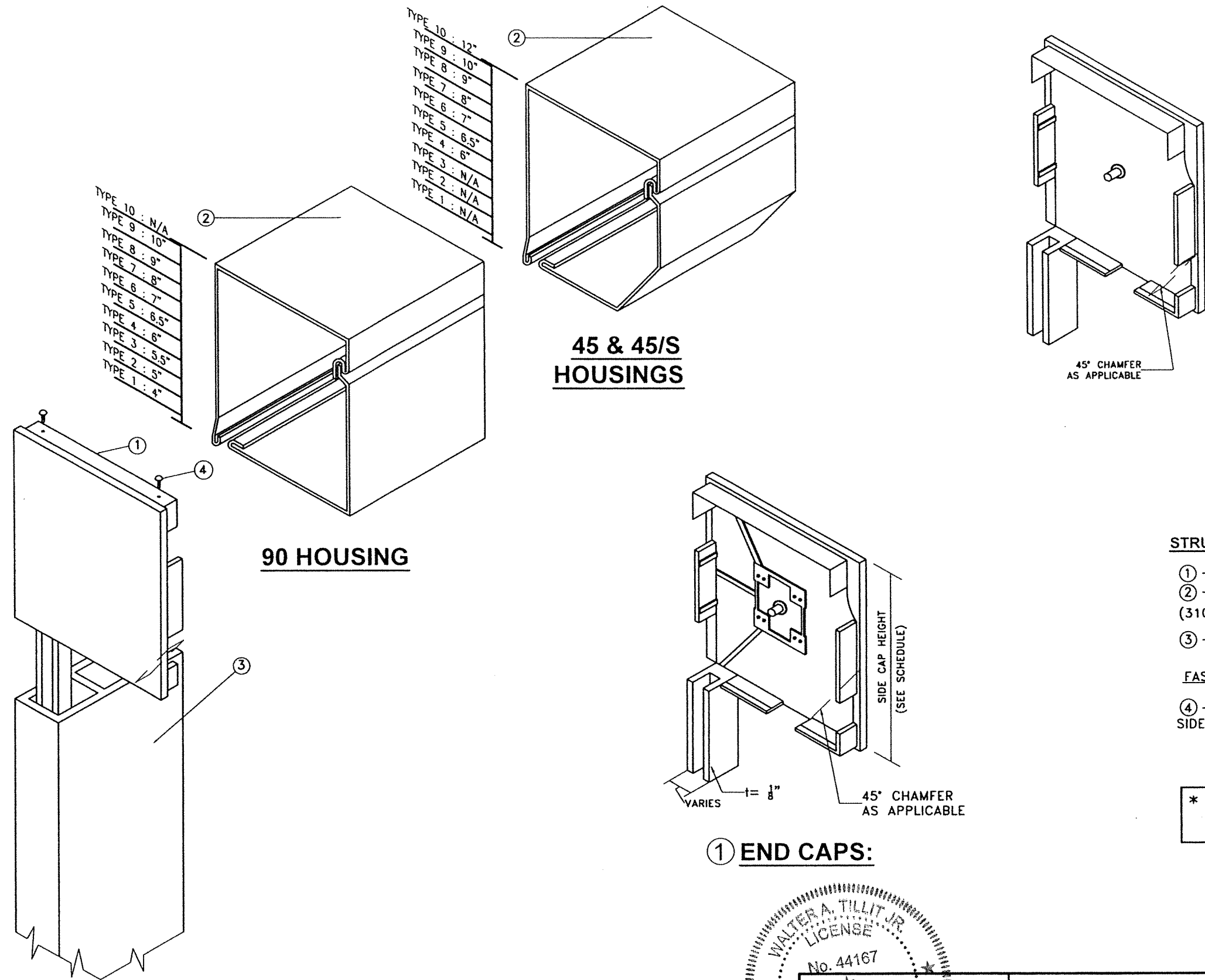
BOX STRUCTURAL COMPONENTS AND ASSEMBLY DETAIL
