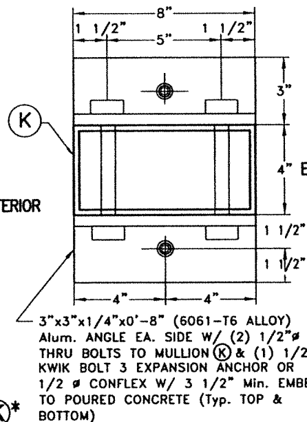
ALTERNATIVES SECTION X1-X1 W/ (K)* (W/ ORIENTATION # 2) (4"x8")
