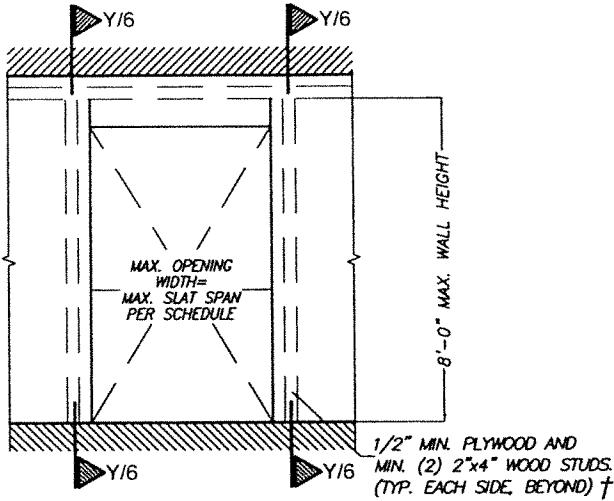
DETAIL 1 (ELEVATION)
