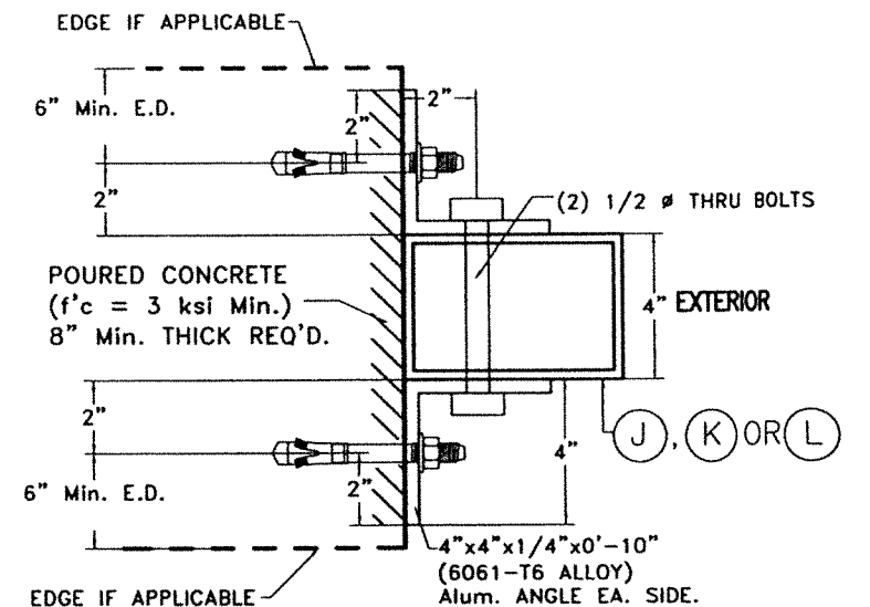
ALTERNATIVE SECTION X2-X2 W/ (J), (K) or (L)* (END & INTERIOR MULLION (J), (K) or INTERIOR MULLION (L) (W/ ORIENTATION # 1) (4"x6", 4"x8" or 4"x4")
