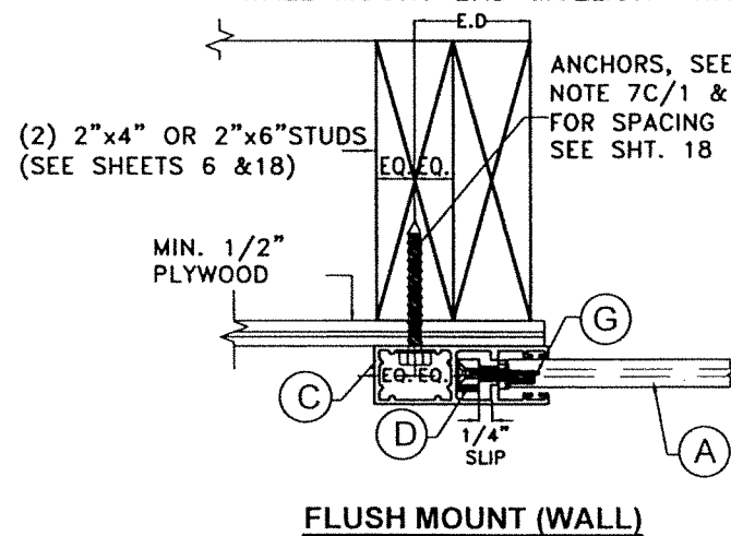
SECTION Q-Q (PLAN) ORIENTATION #1 & #2 WALL MOUNT END MULLION
