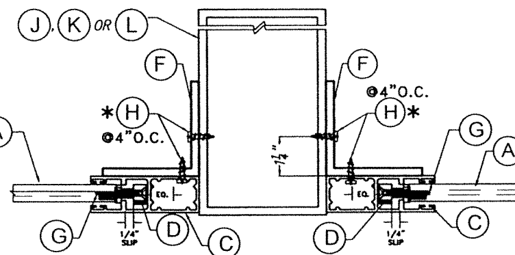
SECTION R'-R' (PLAN) ORIENTATION #1 TRAPPED MOUNT INTERIOR MULLION
