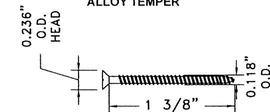
(G) END RETENTION SCREW AT EACH (D) 0.118" O.D. x 1 3/8" AISI 304 STAINLESS STEEL W/ XYLAN COATING
