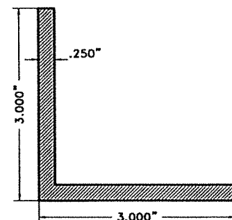
(F) TRAPPED ANGLE 6063-T6 ALUMINUM ALLOY TEMPER
